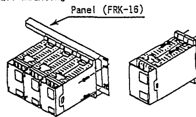
Fig.2 Wall Mounting
